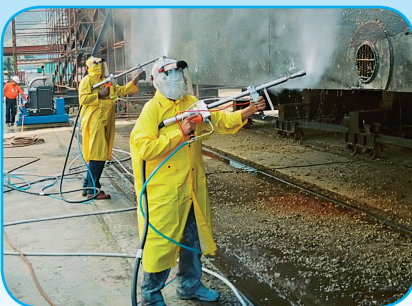
Twin gun surface preparation
